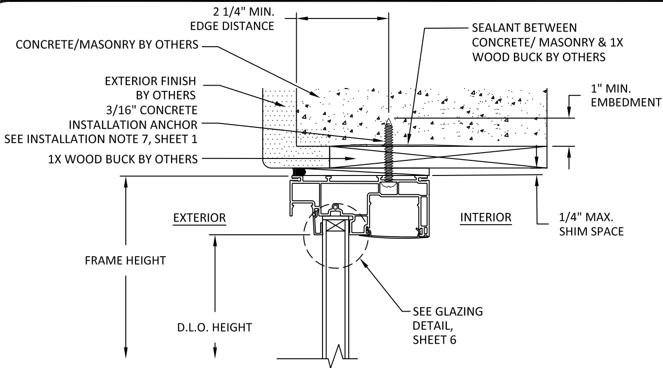
A 4 VERTICAL SECTION THROUGH FRAME INSTALLATION CONCRETE/CMU SUBSTRATE
