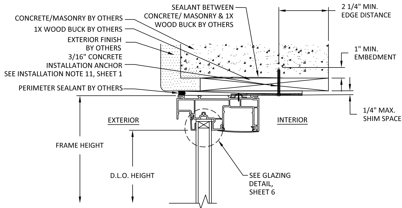
A 5 VERTICAL SECTION CLIP INSTALLATION CONCRETE/CMU SUBSTRATE
