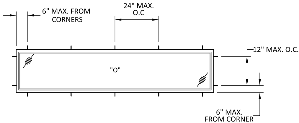
TYPICAL ANCHOR LAYOUT THROUGH FRAME/CLIP INSTALLATION
