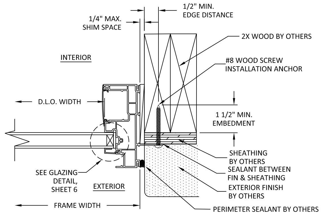
C 3 HORIZONTAL SECTION NAIL FIN INSTALLATION WOOD SUBSTRATE
