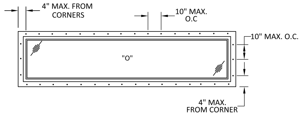
TYPICAL ANCHOR LAYOUT NAIL FIN INSTALLATION
