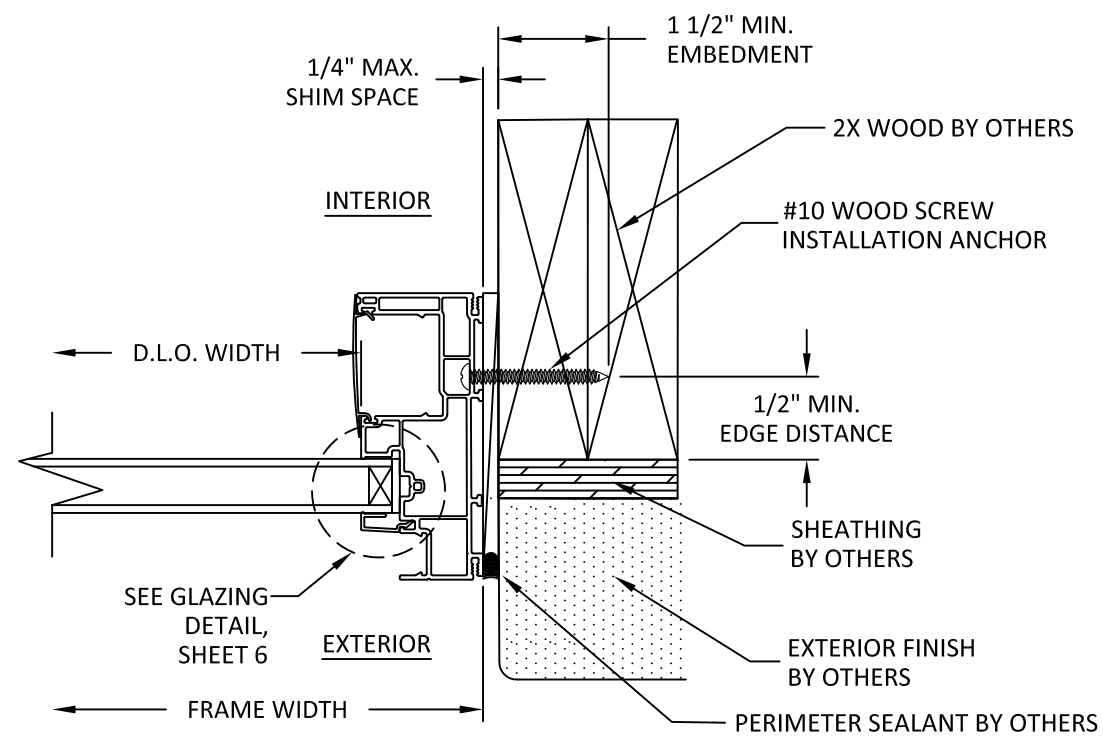
C 4 HORIZONTAL SECTION THROUGH FRAME INSTALLATION WOOD SUBSTRATE
