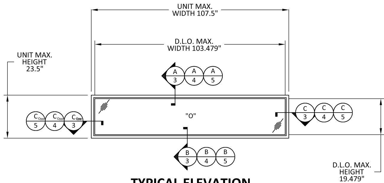
TYPICAL ELEVATION 800 DOOR TRANSOM
