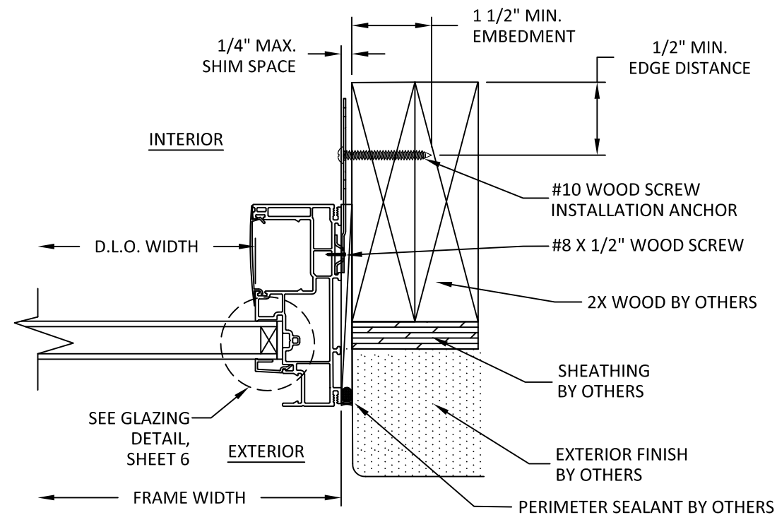
C 5 HORIZONTAL SECTION CLIP INSTALLATION WOOD SUBSTRATE
